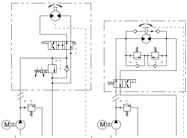
Hydraulic scheme examples
