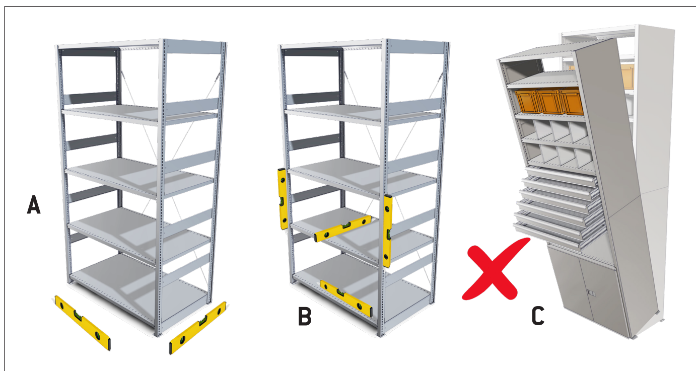
Figura 14 Support floor, levelling and fixing
