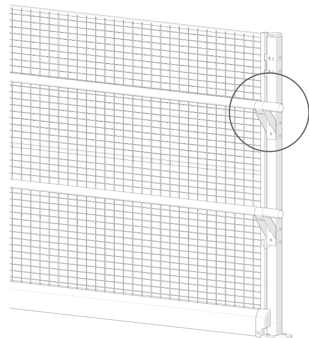
Handrail fittings with rivet, Page : 4
